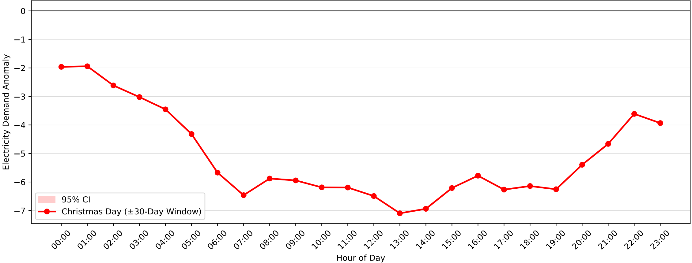
Enfield Demand Anomaly: Christmas Day (2004-2005, \pm 30 -Day Window)
