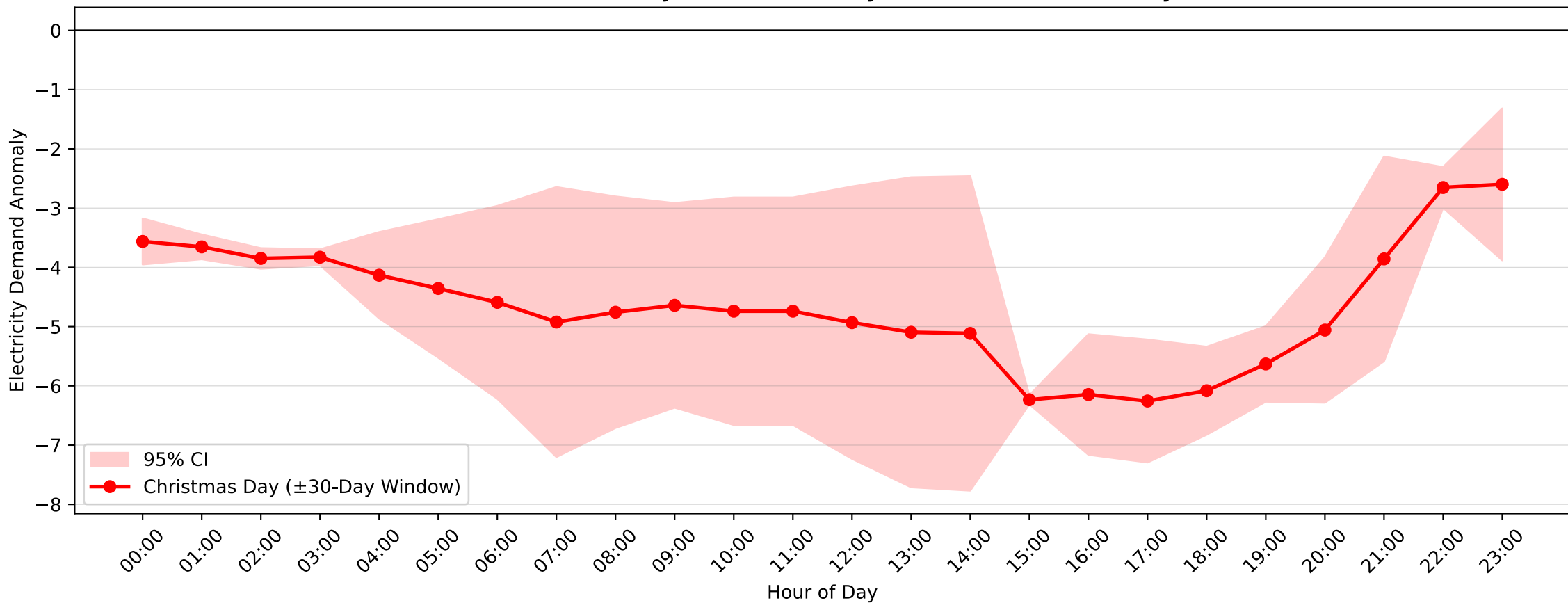
Enfield Demand Anomaly: Christmas Day (2009–2010, \pm 30 -Day Window)
